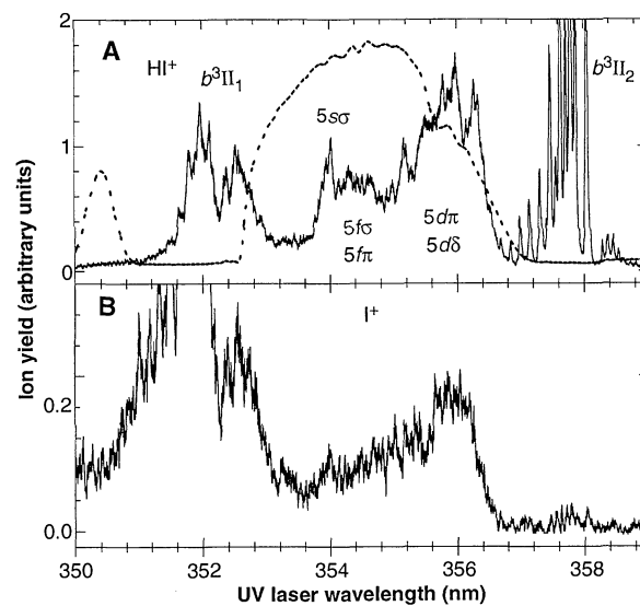
Fig. 4. Photoionization spectrum of HI obtained by adding 12 torr of Xe to the frequency-tripling cell. This spectrum is the sum of both the UV- and VUV-generated signals. The autoionization structure of HI between 353.8 and 356.2 nm is visible in both the (A) HI + and (B) I + data. The dashed line shows the THG efficiency in Xe.
