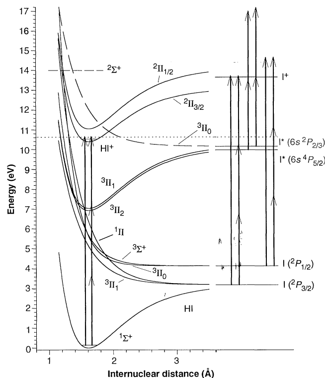
Fig. 1 (left). The UV photoionization spectrum of HI. (A) The \text{HI}^+ signal, including two-photon resonance-enhanced ionization from two of the b^3\Pi , Rydberg states. (B) The \text{I}^+ signal, with strong enhancement of the ion yield in the vicinity of the b^3\Pi , HI resonance. The ionization thresholds of HI and \text{I}(^2P_{3/2}) by three UV photons are indicated with arrows. Fig. 2 (right). Potential energy diagram for HI and I, obtained from (15–18). The short and long arrows on the left indicate the mechanism for controlling the excitation of HI. The arrows on the right indicate possible schemes for ionizing the iodine fragment. The horizontal dotted line corresponds to the energy of three 354.98-nm photons at which one of the phase-control experiments was performed.
