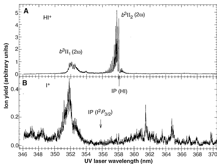
Fig. 1 (left). The UV photoionization spectrum of HI. (A) The \text{HI}^+ signal, including two-photon resonance-enhanced ionization from two of the b^3\Pi , Rydberg states. (B) The \text{I}^+ signal, with strong enhancement of the ion yield in the vicinity of the b^3\Pi , HI resonance. The ionization thresholds of HI and \text{I}(^2P_{3/2}) by three UV photons are indicated with arrows. Fig. 2 (right). Potential energy diagram for HI and I, obtained from (15–18). The short and long arrows on the left indicate the mechanism for controlling the excitation of HI. The arrows on the right indicate possible schemes for ionizing the iodine fragment. The horizontal dotted line corresponds to the energy of three 354.98-nm photons at which one of the phase-control experiments was performed.
