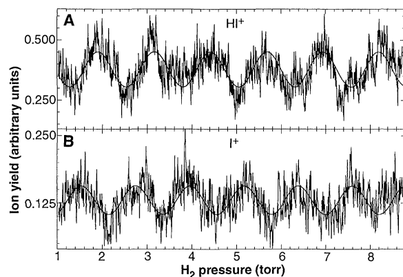
Fig. 3. Modulation of the (A) HI + and (B) I + signals as functions of H 2 pressure in the phase-tuning cell. The HI + signal is seen to lag the I + signal by ~150°. The smooth curves are least-squares fits of the function A + B\cos(cP+d) . The frequency c agrees with the value calculated from the refractive index of H 2 at ω 1 and ω 3 .
