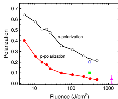
Fig. 1. Polarization of the 460 nm emission vs. laser fluence generated with s-polarized (open symbols) and p-polarized (filled symbols) radiation. The circles are from the present study, the squares are from Majd et al. (Ref. [5]), and the triangle is from Asgill et al. (Ref. [7]).
