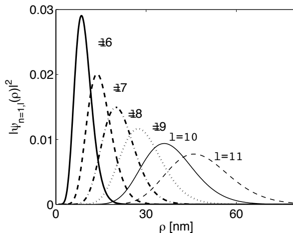
Fig. 2. The n = 1 wave functions (squared) for the set of potentials shown in Fig. 1.
