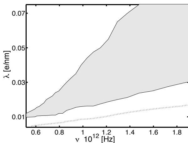
Fig. 5. A stability map of the nano-trap. Trapping exists in the shaded area. The dotted line marks the lower border of the stability region when the contribution of the image potential is removed from the Hamiltonian. This removal has no effect on the upper border line.
